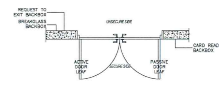
COMPOSITE DRAWING DETAIL FOR DOUBLE DOOR TYPE-1 SCALE: N.T.S.
