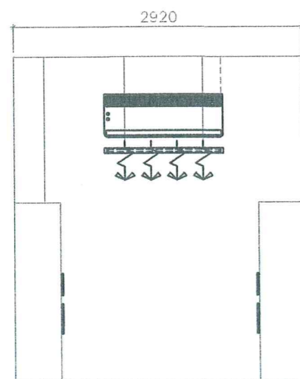
J ELEVATION ID-10 SCALE NTS.
