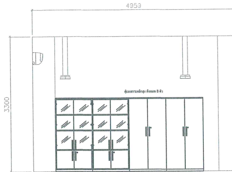
I ELEVATION ID-10 SCALE NTS.
